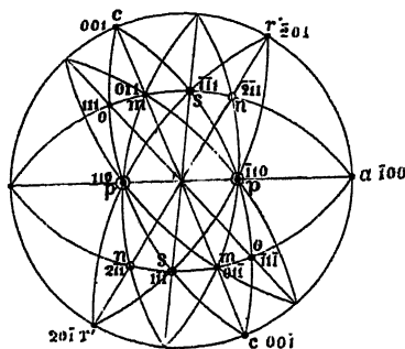
FIG. 108.—Stereographic Projection of Calcium Dextro-Glycerate.
